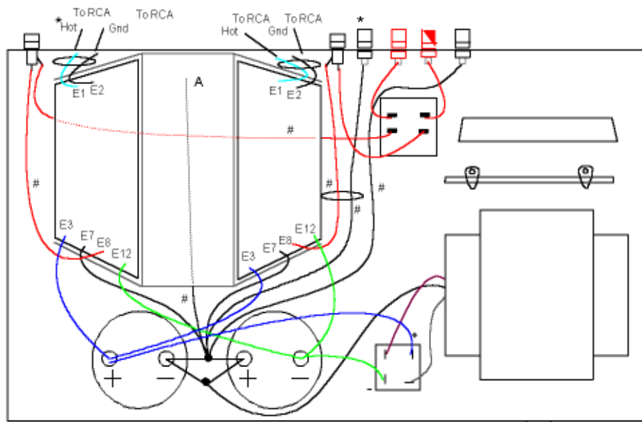
DH-500 BASIC LAYOUT
