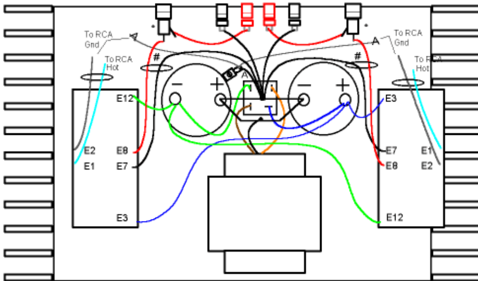
Fig. B DH-200/220 BASIC LAYOUT
